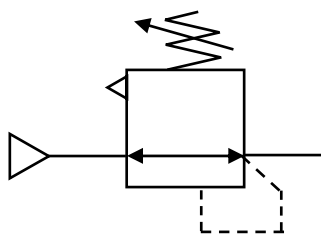
Pressure Regulator Adjustable – Spring Loaded Self-relieving
